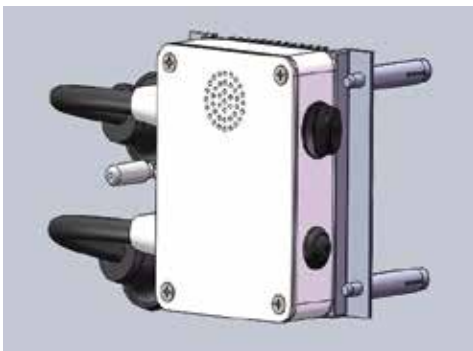
Figure1:Fix the control IHBD3 on the wall first.
